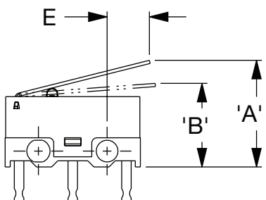
L21 LEVER 14MM
