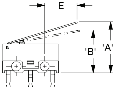
L21 LEVER 14MM
